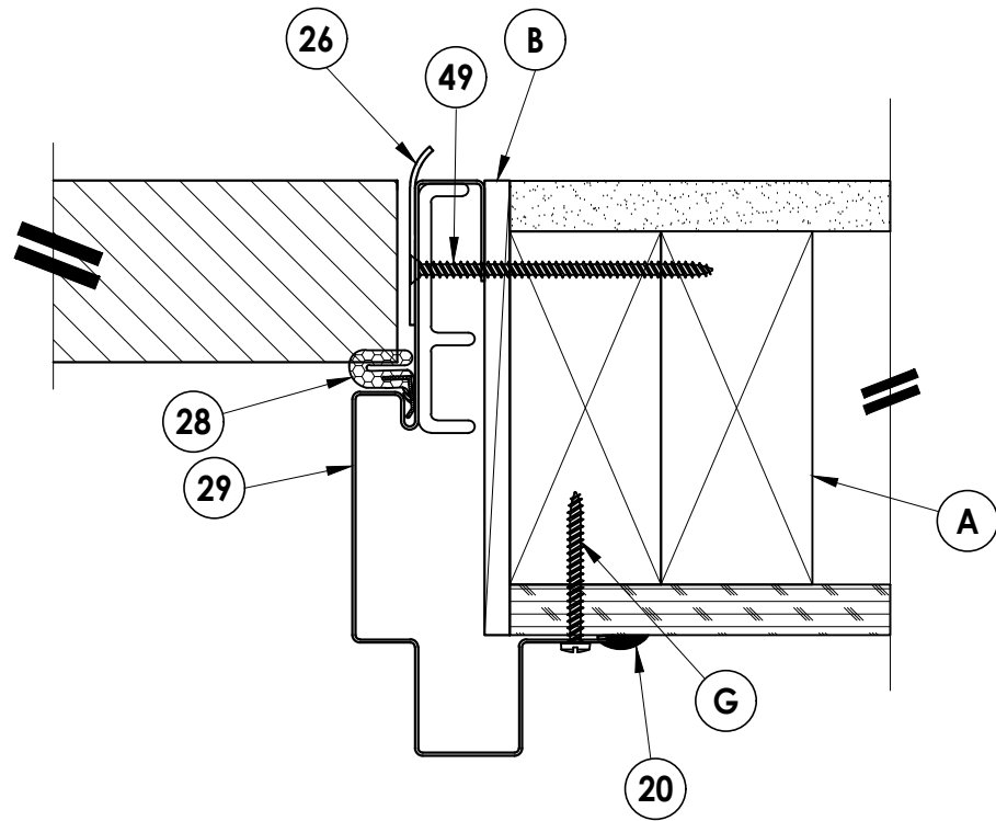
2 6 HORIZONTAL CROSS SECTION 2X Masonry construction
