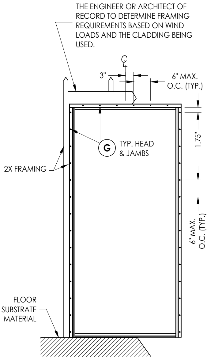
FRAME ANCHORING STUD CONSTRUCTION
