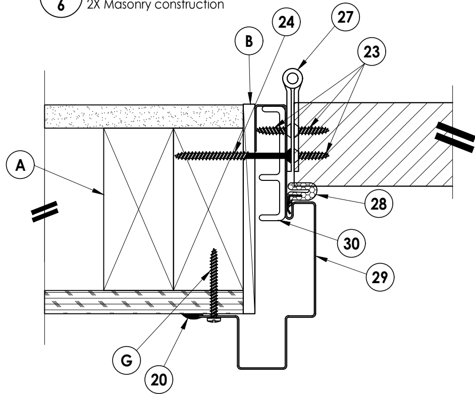
3 6 HORIZONTAL CROSS SECTION 2X Stud construction
