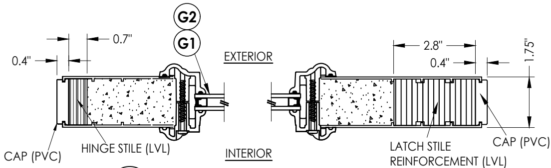
1/4 HORIZONTAL CROSS SECTION
