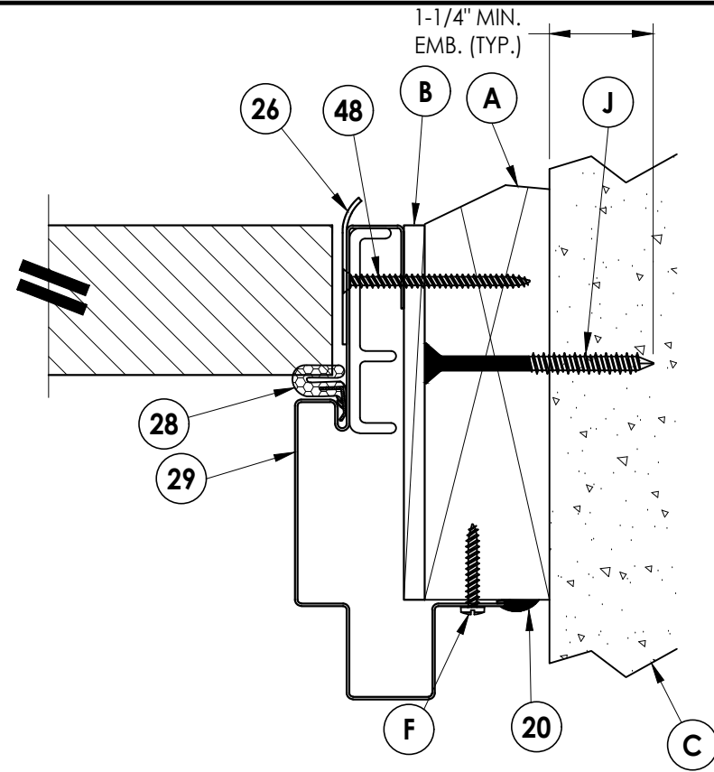
2 6 HORIZONTAL CROSS SECTION 2X Masonry construction
