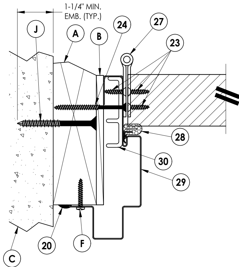
1 6 HORIZONTAL CROSS SECTION 2X Masonry construction
